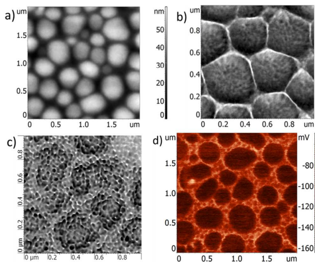
Fig. 1. PTB7:PC 71 BM blend films with no additive (Sample 1): a) Topography measured with AFM, b) Hard-tapping AFM phase image, where repulsive tip-sample forces dominate, enabling observation of a sub-structure inside the domains. c) After removing a top layer of the sample with plasma etching, AFM phase images show the sub-structure more clearly.
